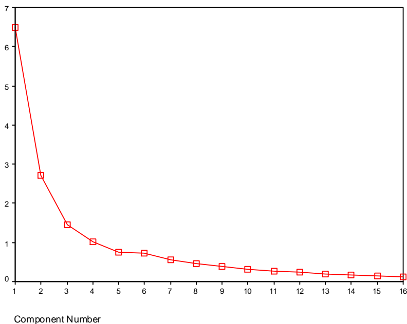
Scree Plot
